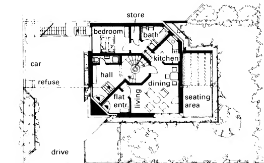
9 Ground floor with self-contained flat → 7 + 8
